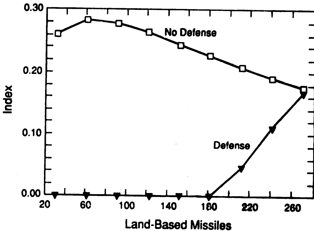
Fig. 4. Strike index
